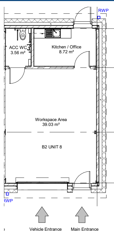
Floor plan example (Unit 9)
